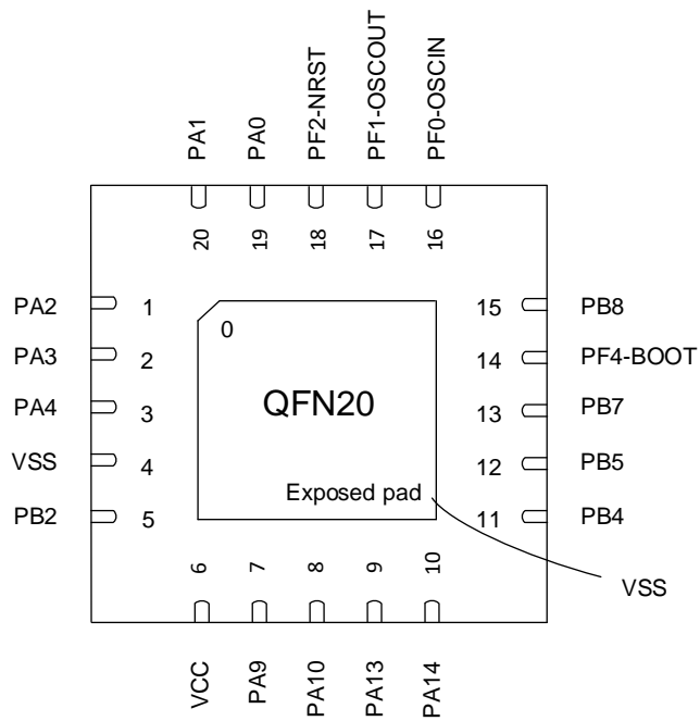
图 3-9 QFN20 Pinout1 PY32F030F1xU
