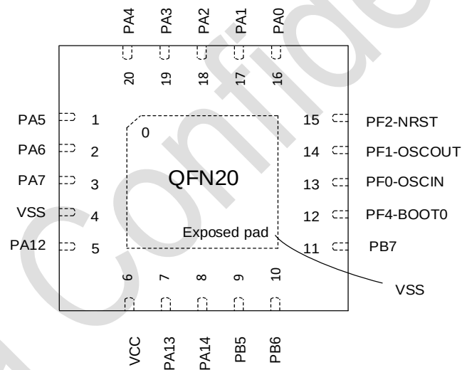
图 3-10 QFN20 Pinout2 PY32F030F2xUx / PY32F030F2xUx-E (Top view)
