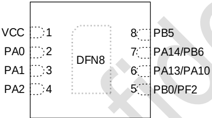
图 3-16 DFN8(1.5*1.5) Pinout1 PY32F030L1xDx (Top view)
