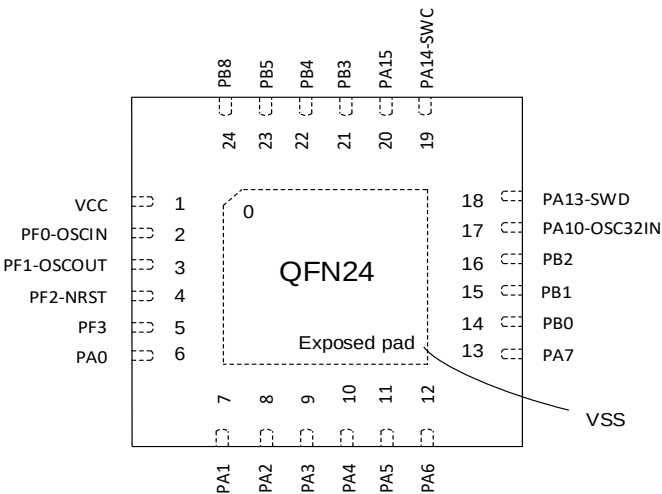
图 3-6 QFN24 Pinout1 PY32F030E1xUx-E (Top view)
