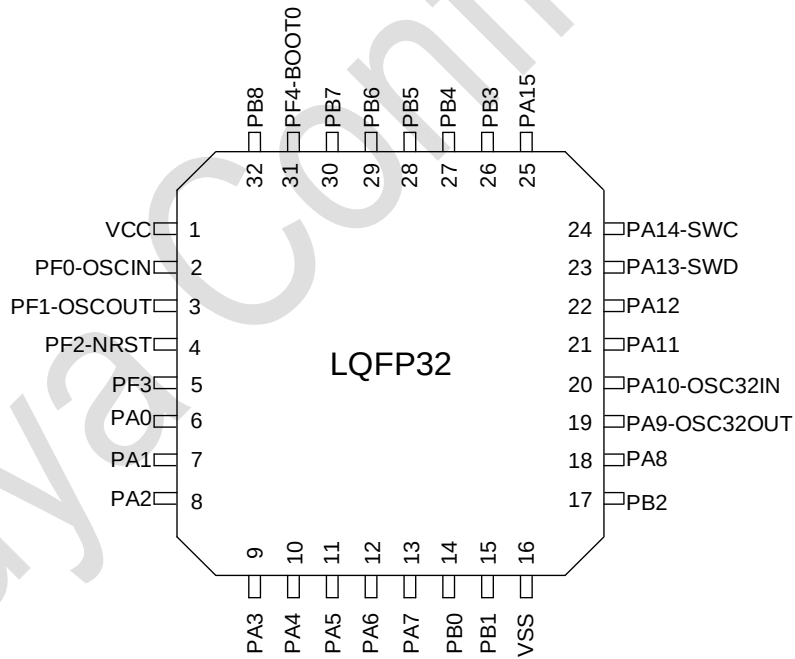
图 3-2 LQFP32 Pinout2 PY32F030K2xTx / PY32F030K2xT-E (Top view)
