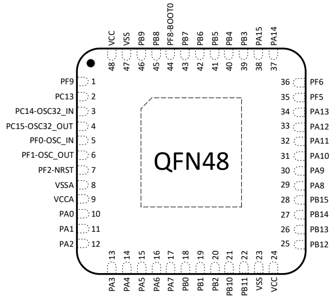
图 3-3 QFN48 PY32F040C1xU Pinout1
