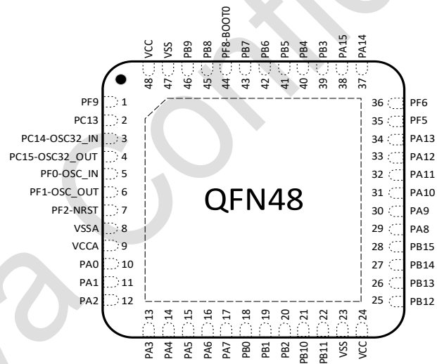
图 3-4 QFN48 PY32F072C1xU6 Pinout1 (Top view)
