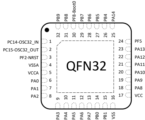
图 3-5 QFN32 PY32F072K1xU6 Pinout1 (Top view)
