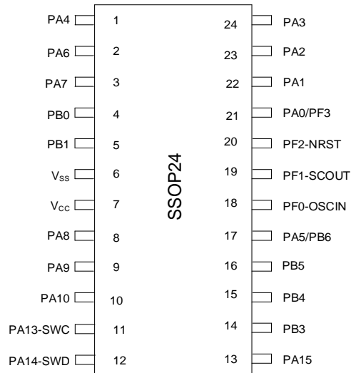
图 3-1 SSOP24 Pinout1 PY32M030E1xM7
