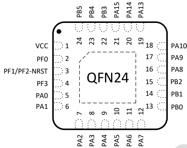
图 3-1 QFN24 Pinout1 PY32M070E1xU7 (Top view)
