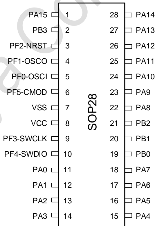
图 3-4 SOP28 Pinout2 PY32T020G2xS7 (Top view)
