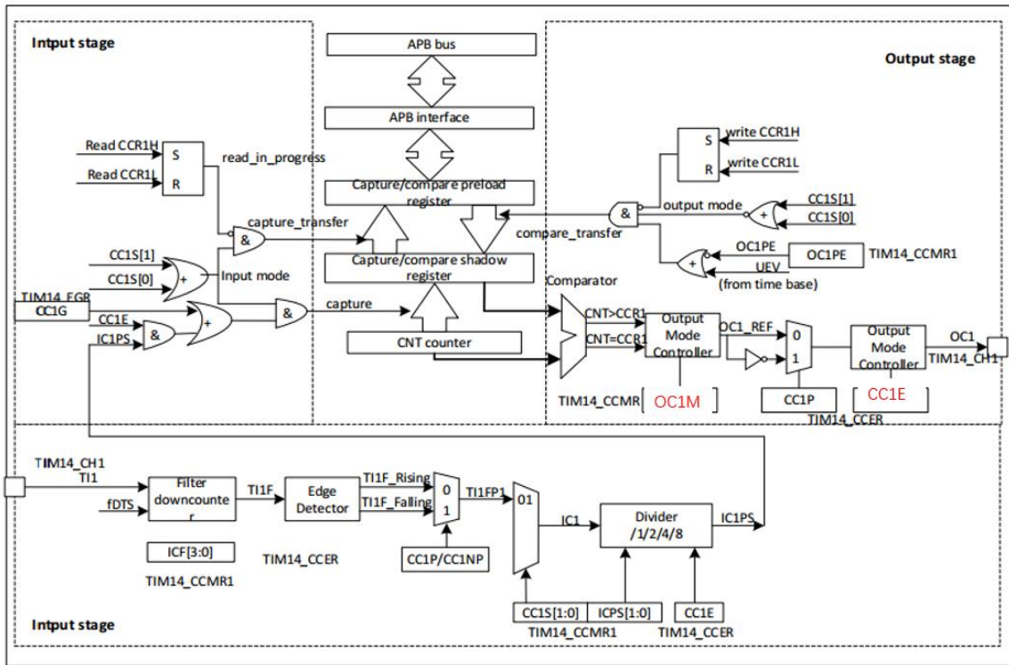
Figure 16-11 Capture/compare channel
