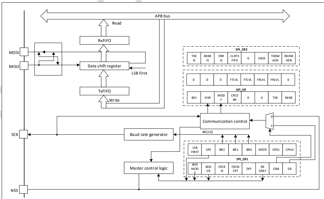
Figure 25-3 SPI Module
