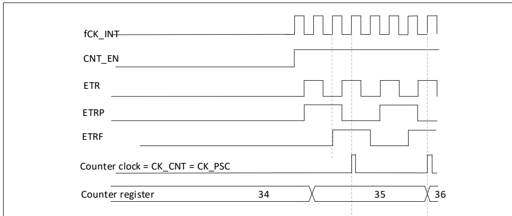
Figure 13-26 Control circuit in external clock mode 2
