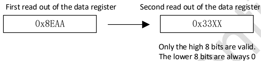
Figure 25-17 Read in receive mode
