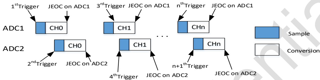
Figure 12-13 Alternate Trigger - Group of Injection Channels per ADC
